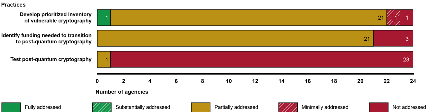
Figure 4: Extent to Which the 24 Chief Financial Officers Act Agencies Addressed Preparatory Practices for Migrating to Quantum Computing
